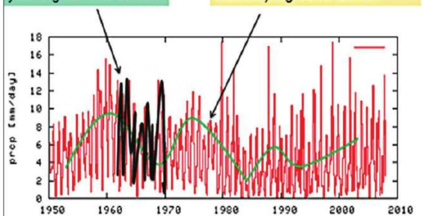
Figure 1. Climate Variability in rainfall: inter-annual and decadal variability. (Source: Taylor 2018.)
