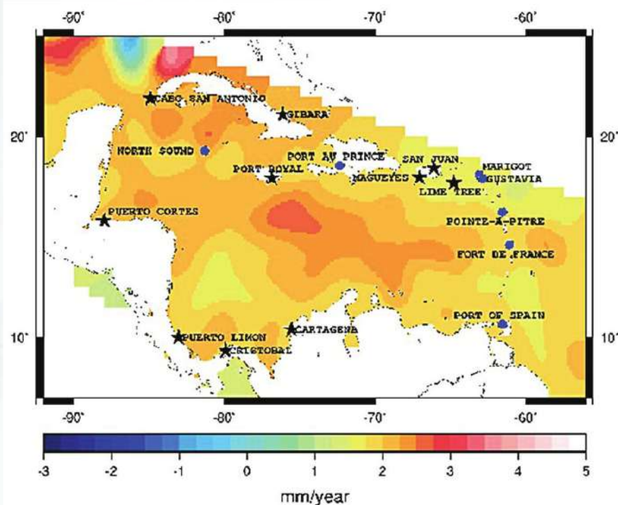
Figure 8. Sea level rise (mm/year) in the Caribbean Mean Reconstruction Sea Level (MRESL)1950- 2009. Palanisamy et al. (2012).
