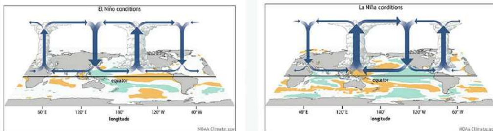
Figure 6. Generalised air circulation and weather conditions associated with (a) El Niño and (b) La Niña conditions
